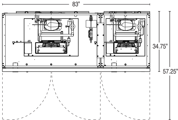
CR3S-FGE (Showing Door Swings)
