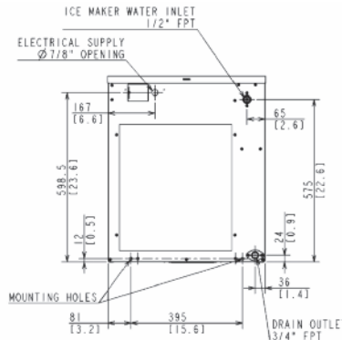
AIR-COOLED UNIT
