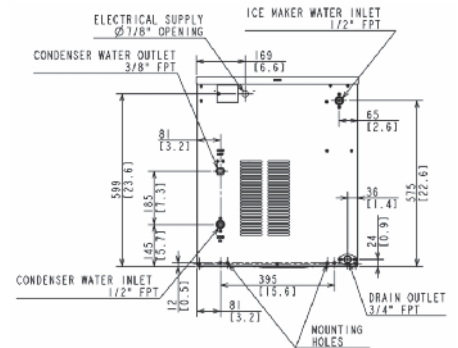
WATER-COOLED UNIT
