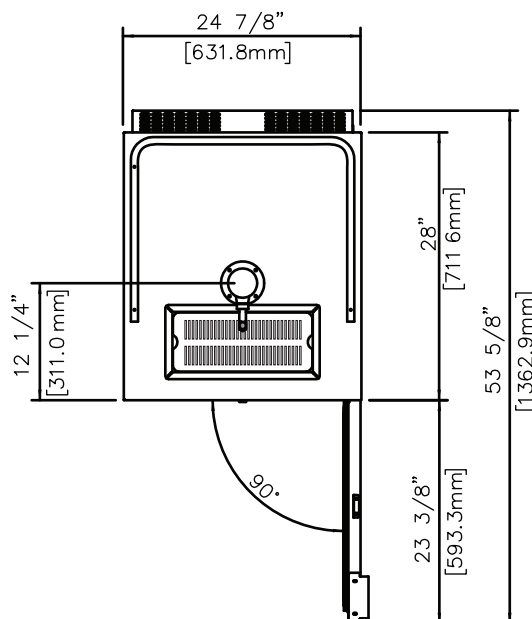
HDD-1-24(-S) Plan View
