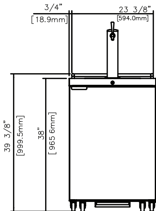
HDD-1-24(-S) Front View
