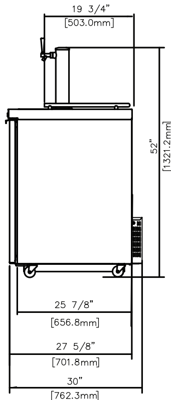
HDD-1-24(-S) Side View
