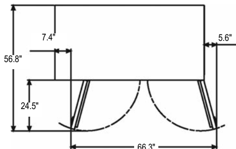
HUR68A (DOOR SWING)
