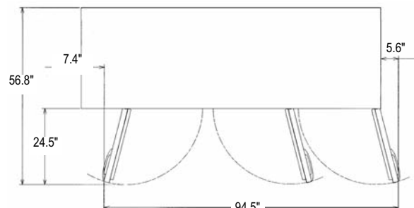
HUR96A (DOOR SWING)
