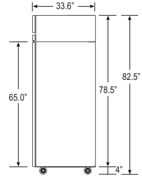
SIDE VIEW (ALL UNITS)
