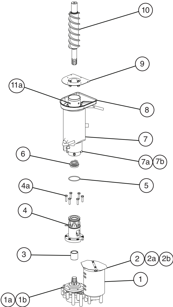
F-822M_K-C, F-1022M_K(Z)(-C)(-CB)
