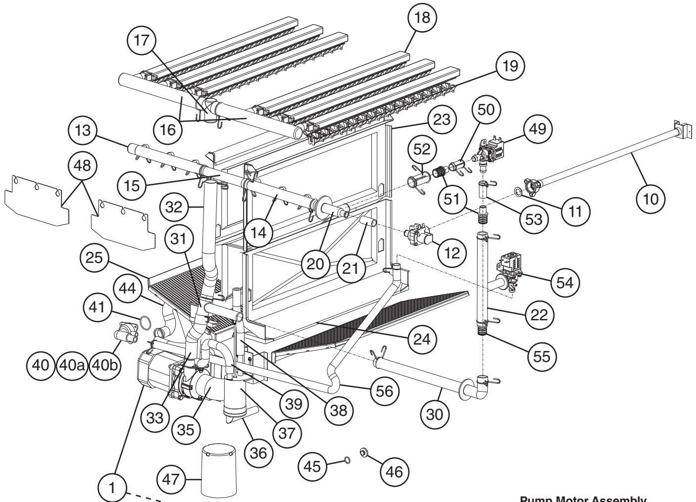
Pump Motor Assembly
