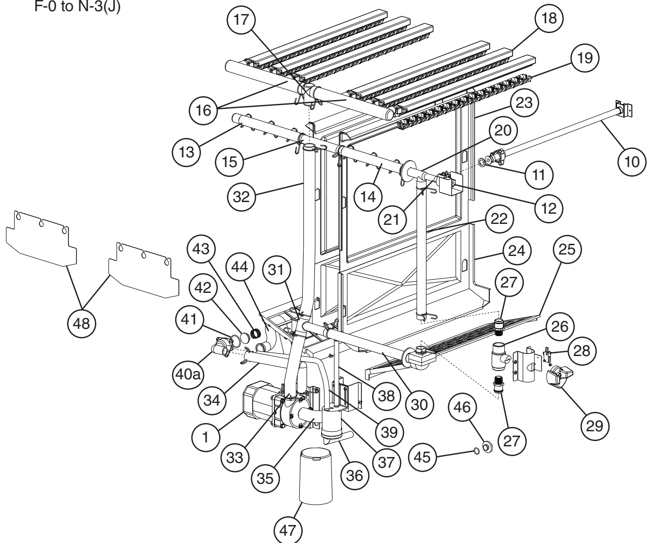
Pump Motor Assembly
