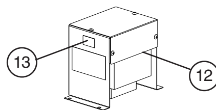
Main Transformer Box Assembly KM-1601SWJ3
