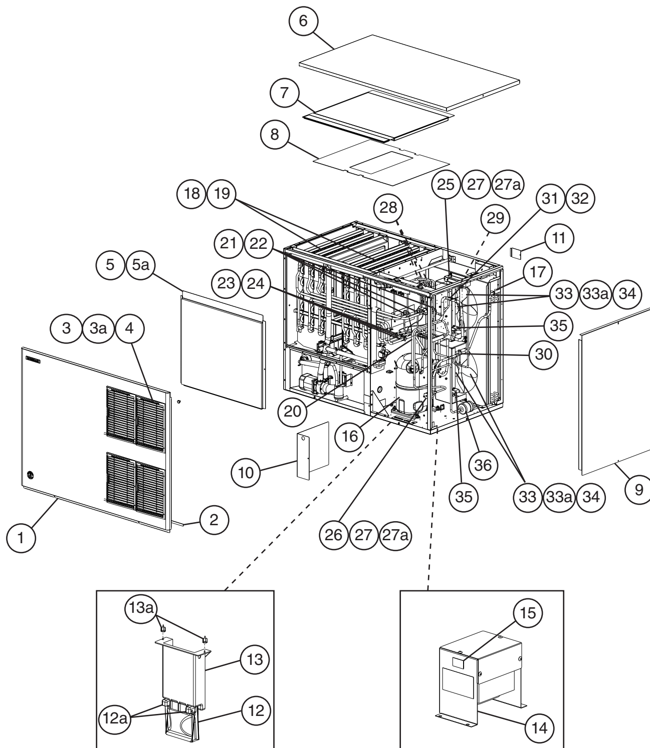
Main Transformer Box Assembly KM-1900SAJ3
