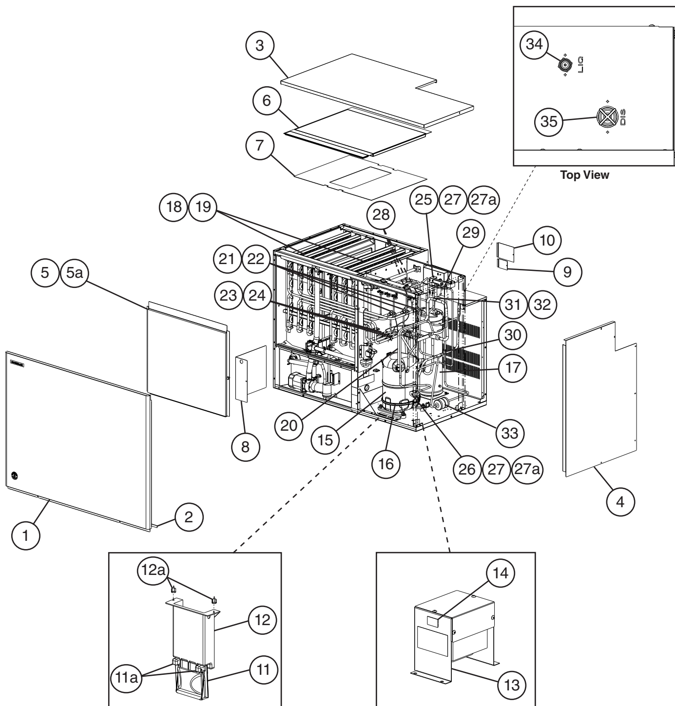
Main Transformer Box Assembly KM-1900SRJ3
